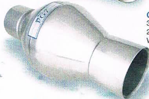
G-19 (65A) 19-core model 140x314mm Water flow 26.0m 3 /h
